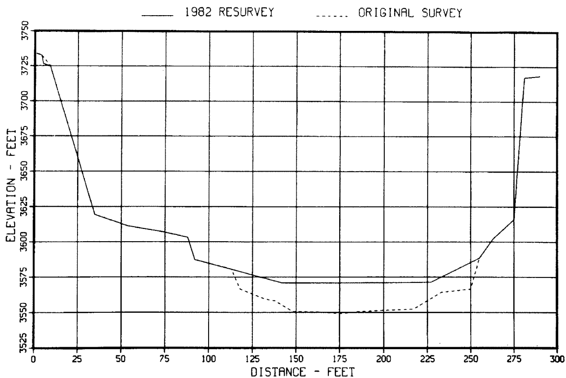
Figure 83. - Original and 1982 sedimentation range profiles, range 101.
