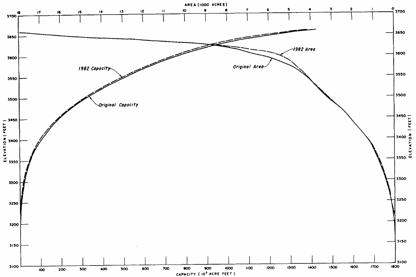
Figure 12. – Area-capacity curve.
