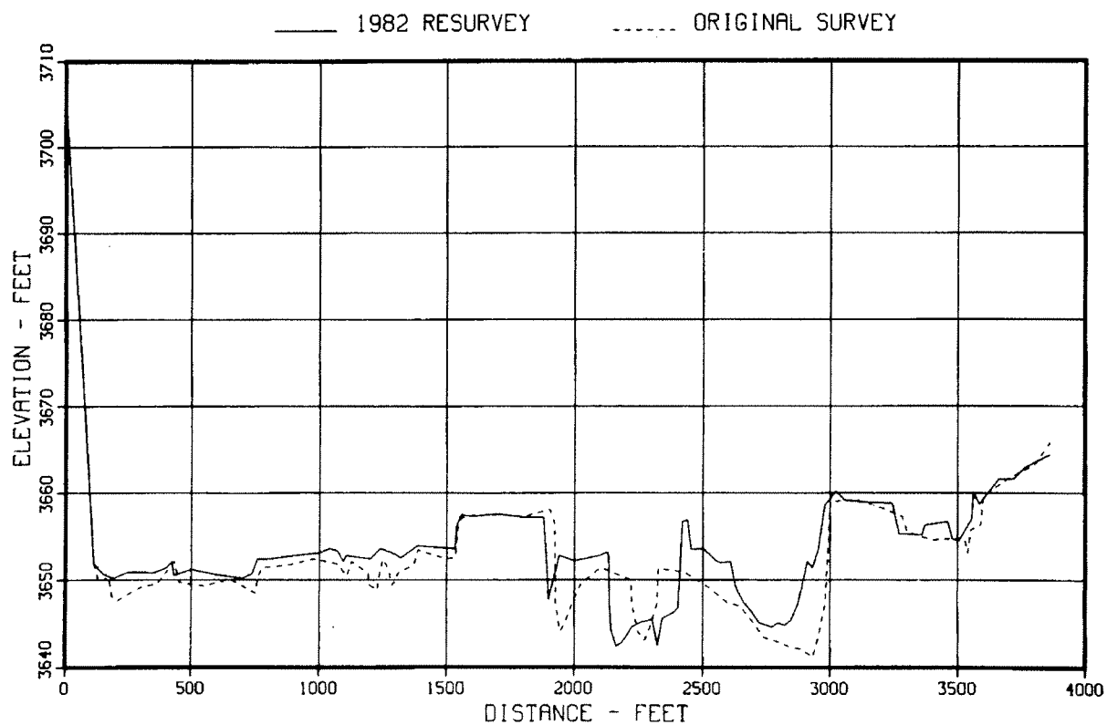
Figure 74. – Original and 1982 sedimentation range profiles, range 40.
