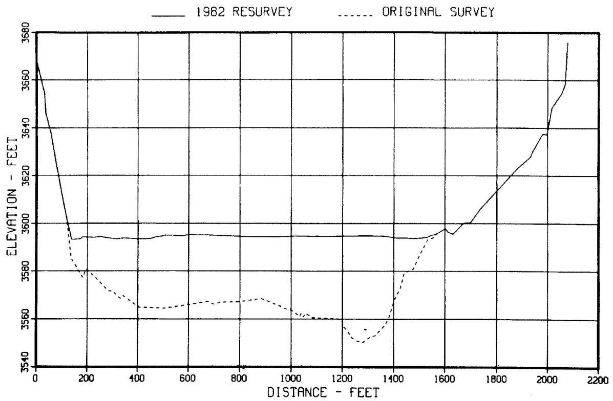
Figure 49. – Original and 1982 sedimentation range profiles, range 15.
