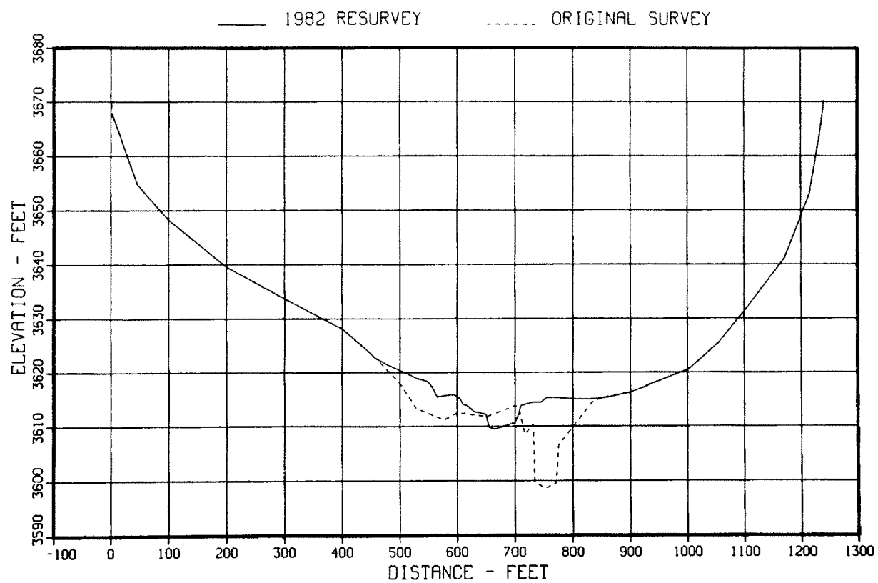
Figure 85. — Original and 1982 sedimentation range profiles, range 103.
