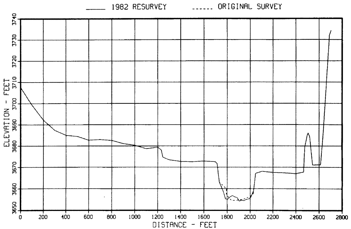
Figure 78. - Original and 1982 sedimentation range profiles, range 44.
