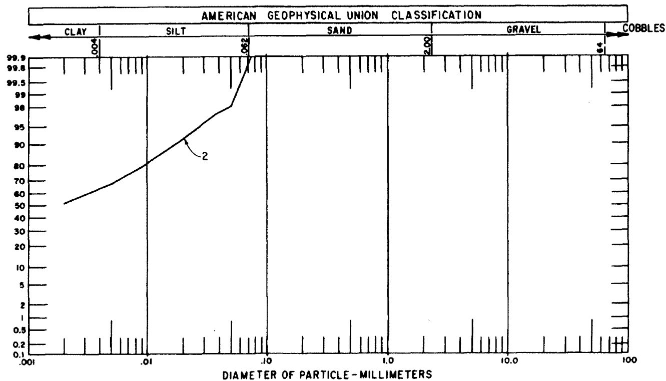
Figure 14. - Particle size analysis curve, range 14.
