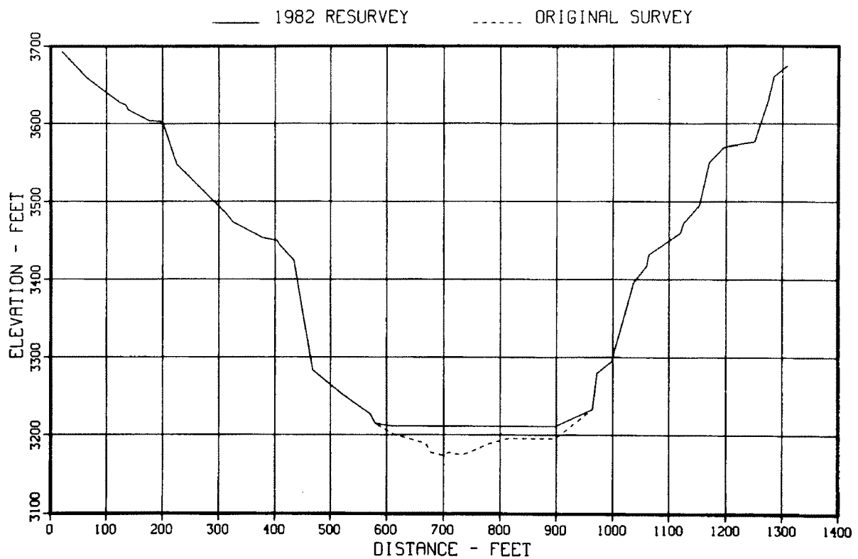
Figure 35. – Original and 1982 sedimentation range profiles, range 1.
