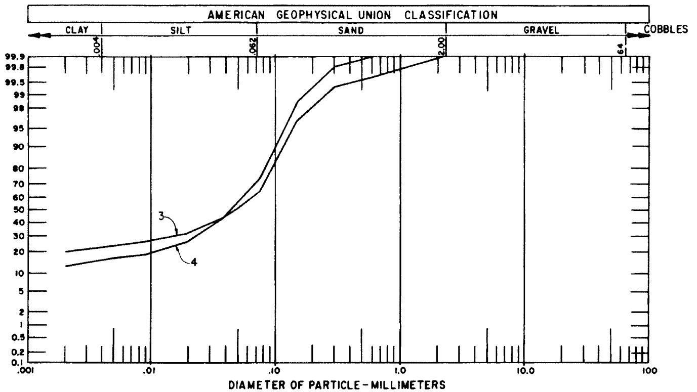
Figure 15. - Particle size analysis curves, range 15.
