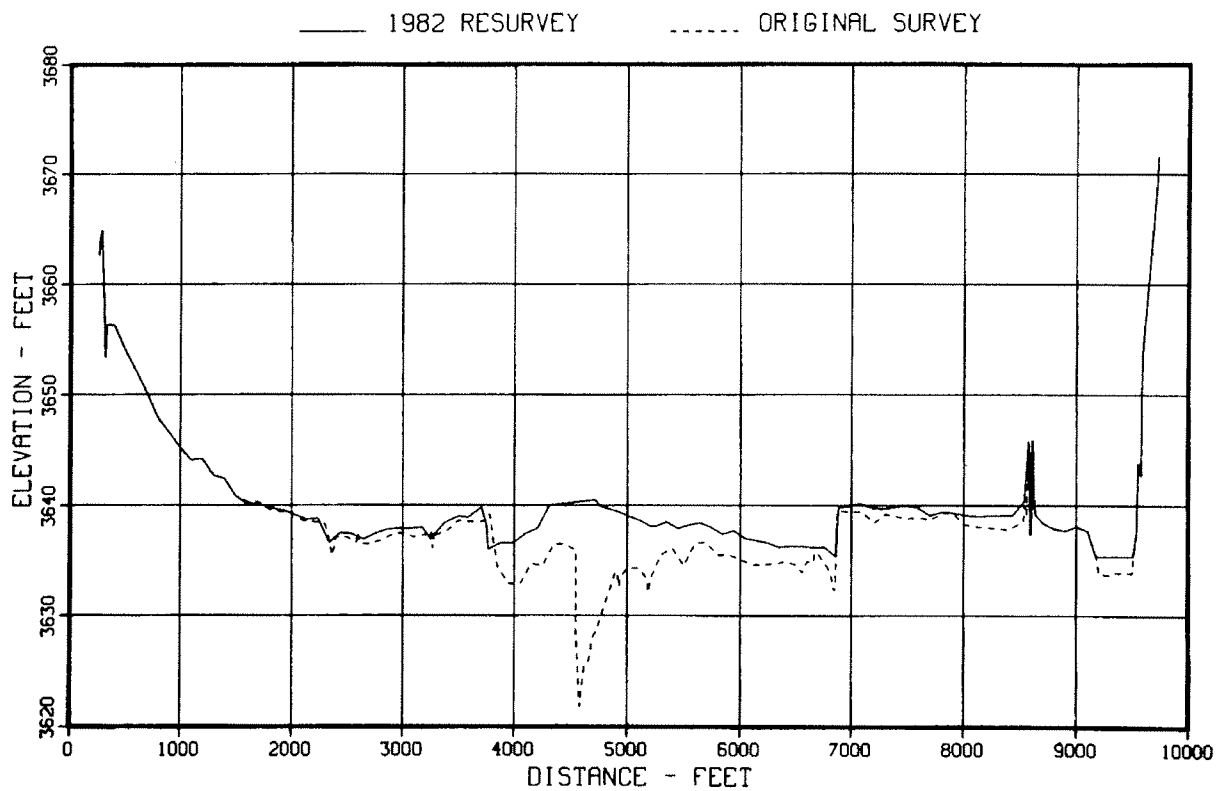
Figure 69. – Original and 1982 sedimentation range profiles, range 35.
