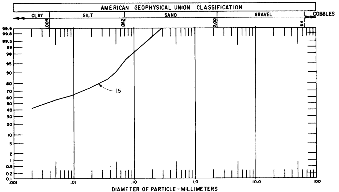
Figure 24. - Particle size analysis curve, range 24.
