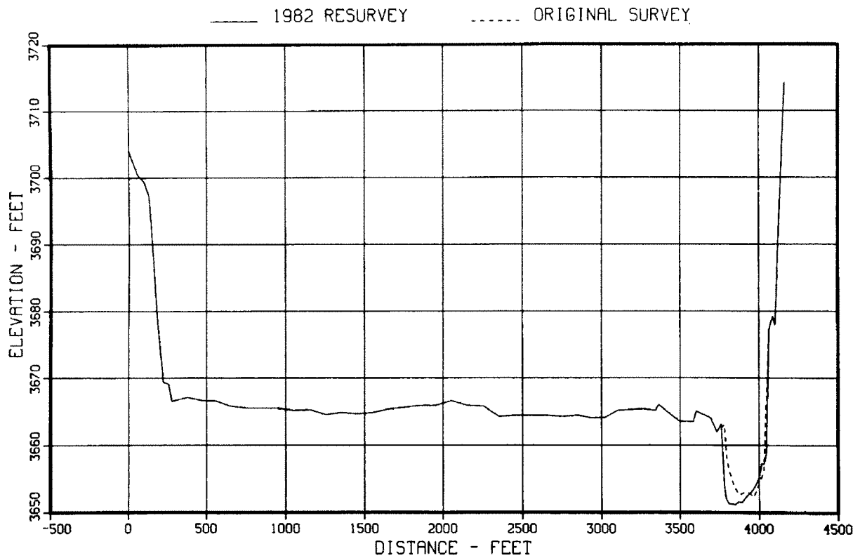
Figure 77. - Original and 1982 sedimentation range profiles, range 43.
