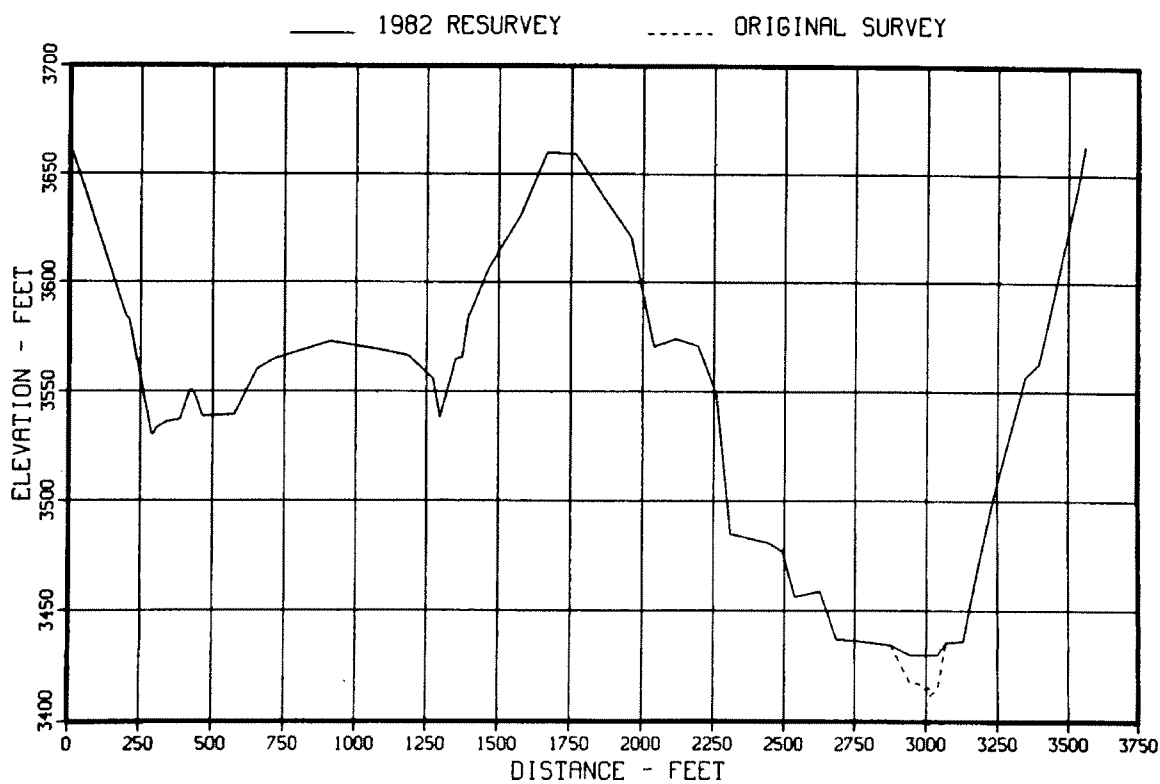
Figure 80. - Original and 1982 sedimentation range profiles, range 3A.
