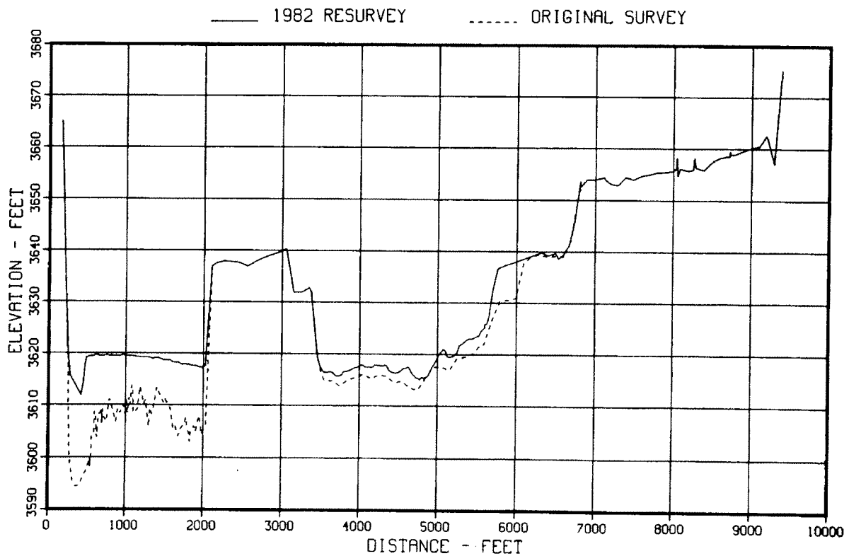
Figure 60. - Original and 1982 sedimentation range profiles, range 26.
