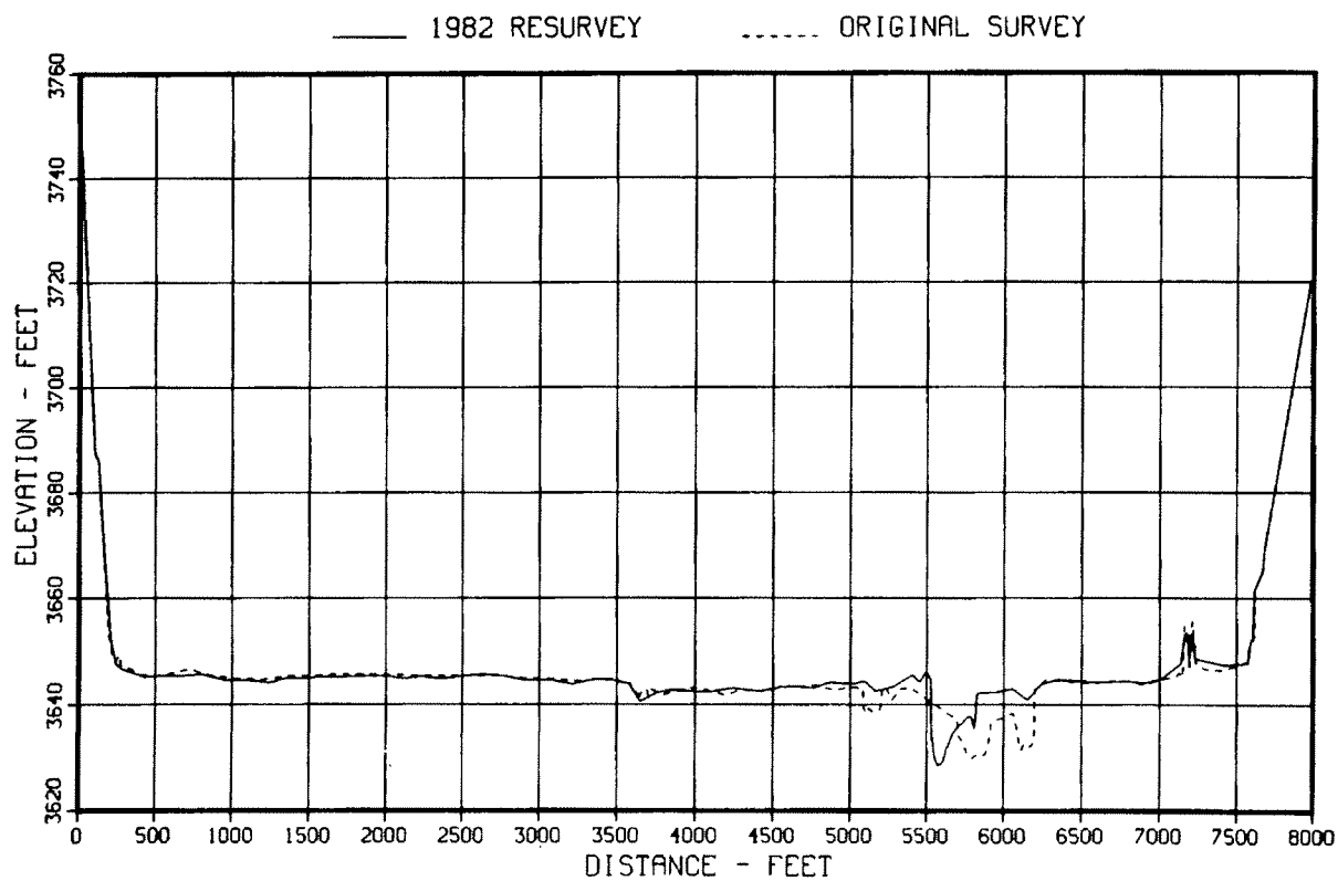
Figure 70. – Original and 1982 sedimentation range profiles, range 36.
