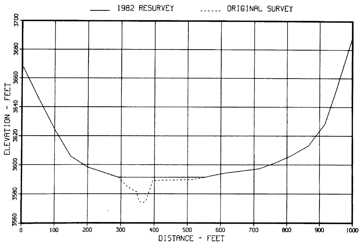
Figure 84. - Original and 1982 sedimentation range profiles, range 102.
