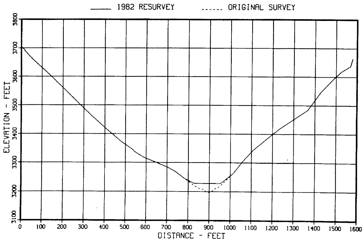
Figure 36. – Original and 1982 sedimentation range profiles, range 2.
