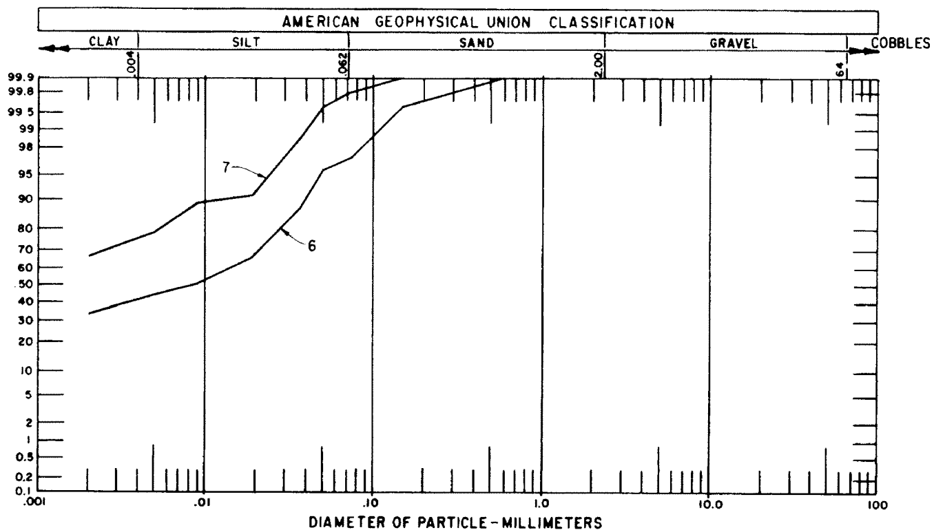
Figure 17. - Particle size analysis curves, range 17.
