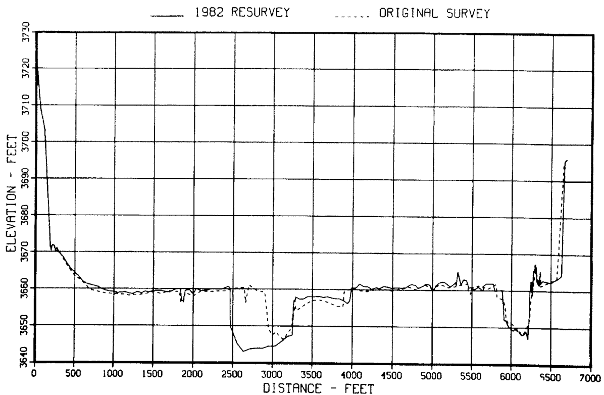
Figure 75. - Original and 1982 sedimentation range profiles, range 41.
