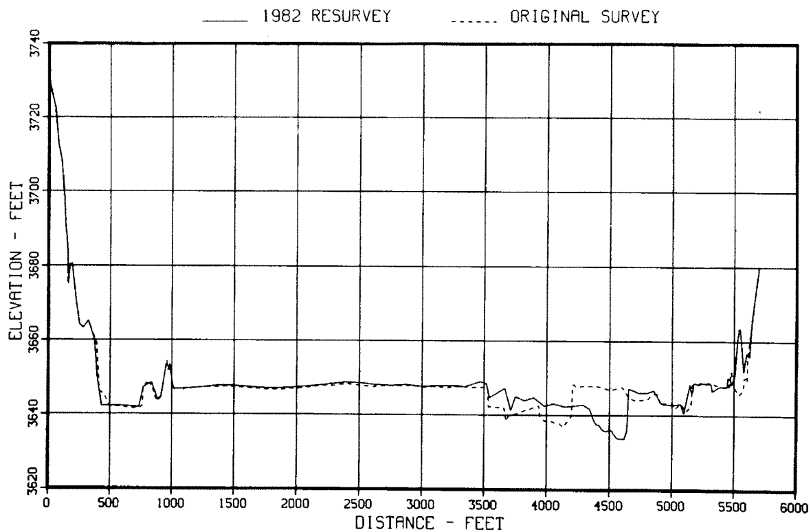
Figure 71. - Original and 1982 sedimentation range profiles, range 37.
