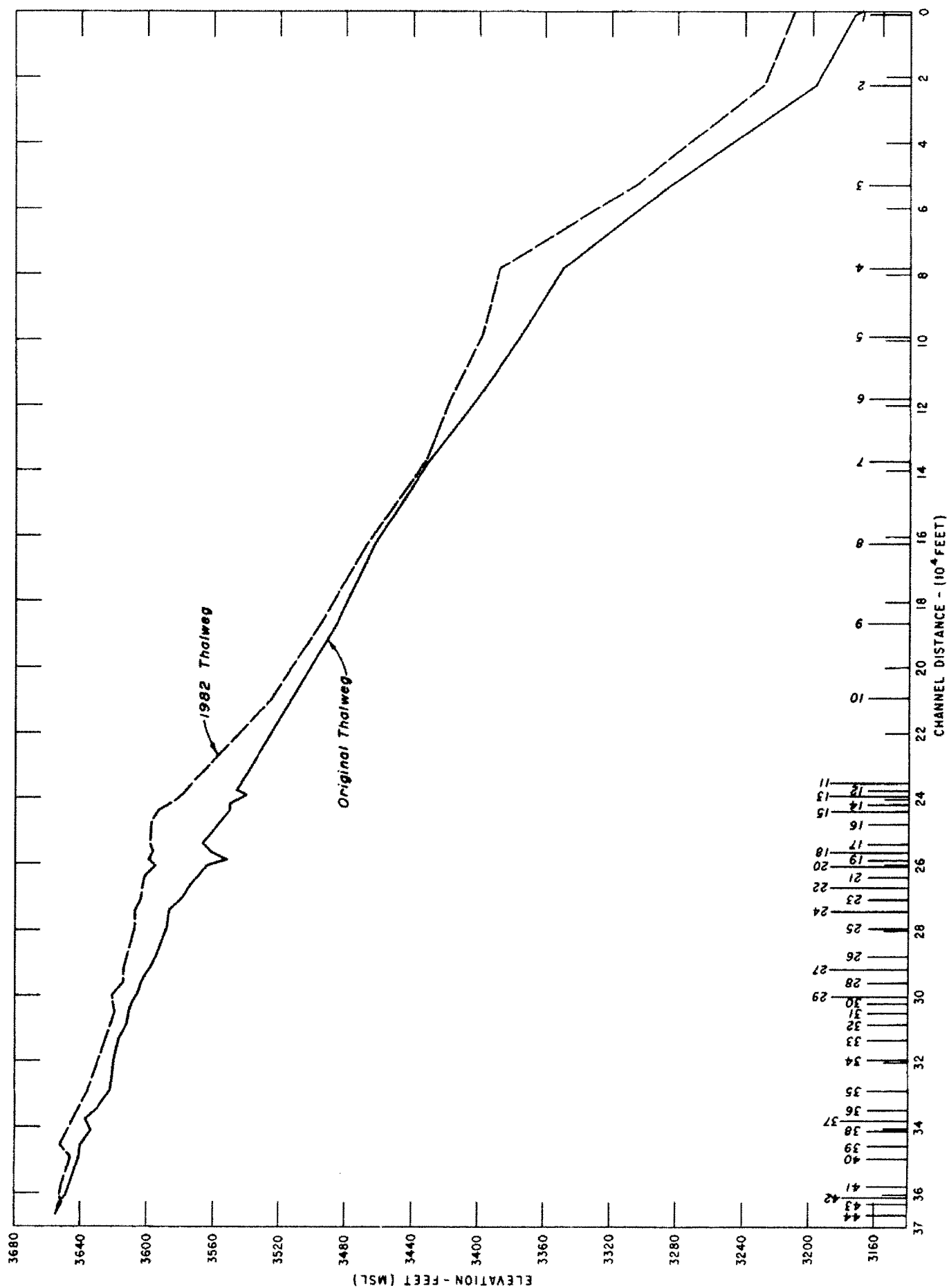
Figure 30. - Longitudinal thalweg profiles for Bighorn Lake.
