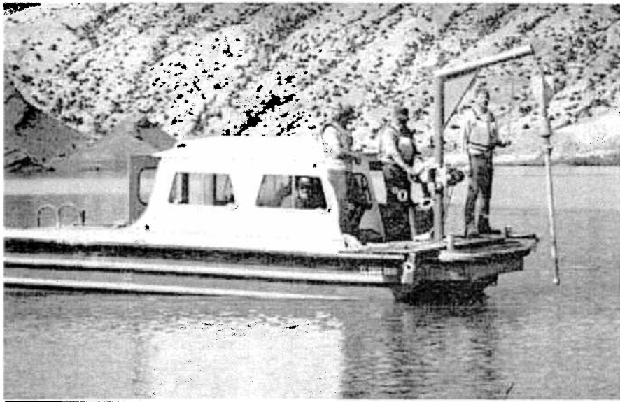
Figure 11. – Gravity core sampler and retrieval system.
