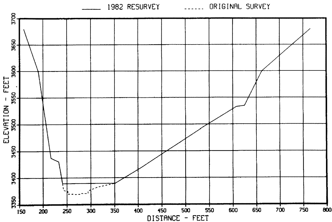
Figure 81. - Original and 1982 sedimentation range profiles, range 4A.
