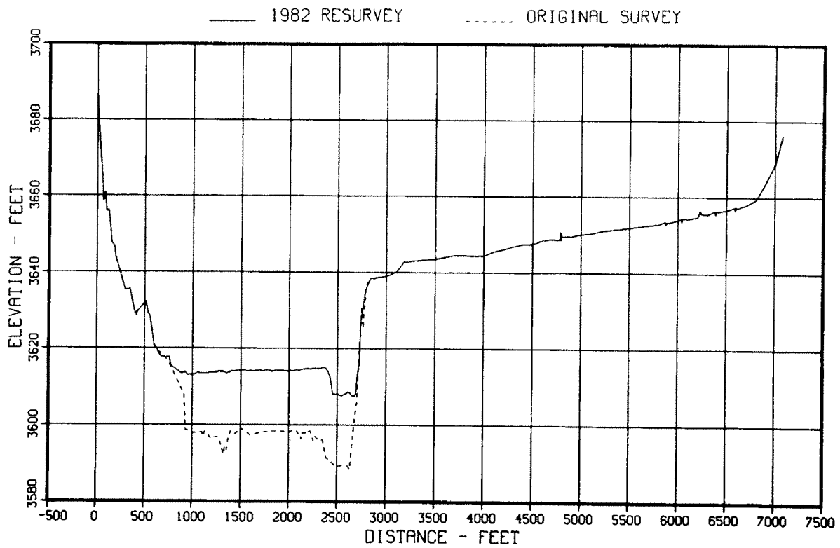
Figure 59. - Original and 1982 sedimentation range profiles, range 25.
