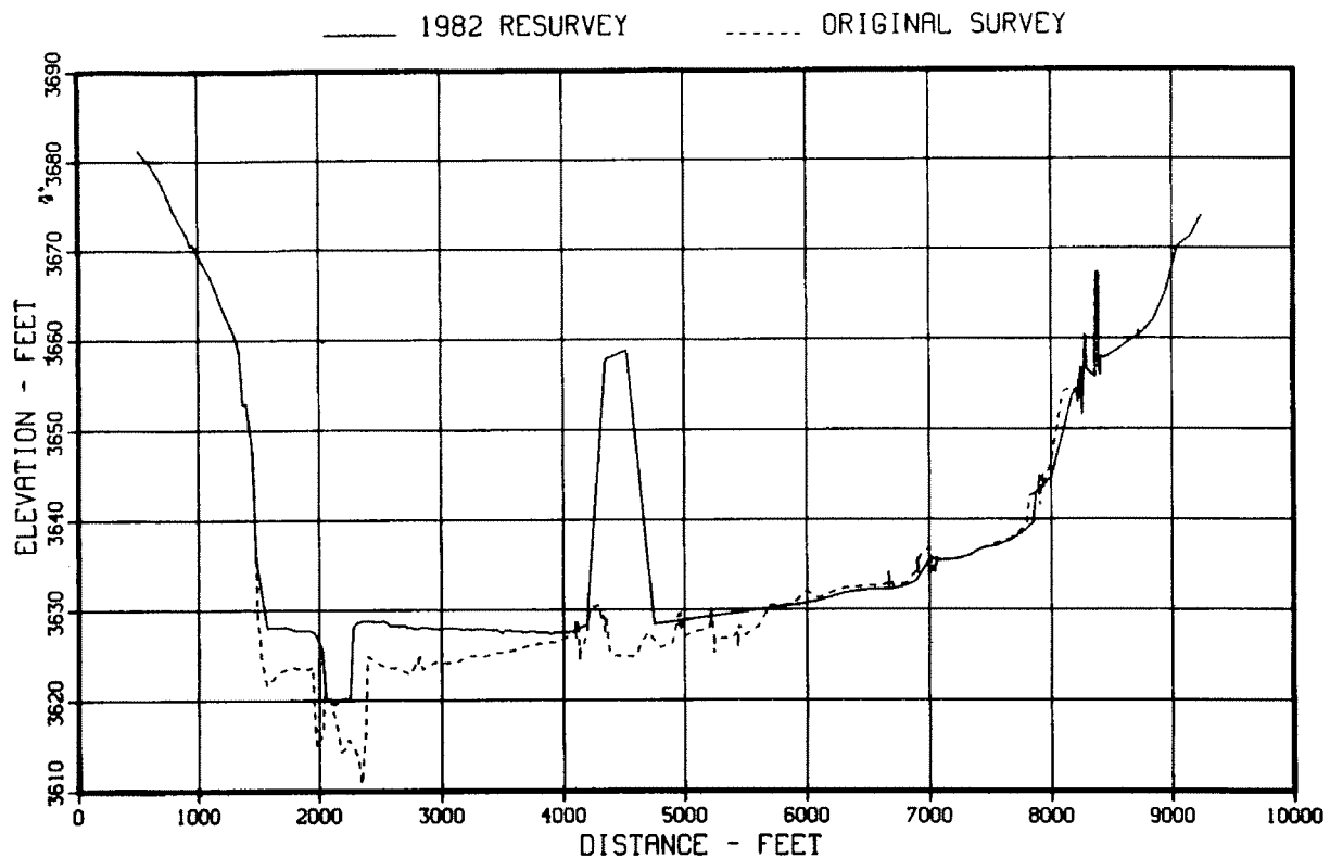
Figure 65. - Original and 1982 sedimentation range profiles, range 31.
