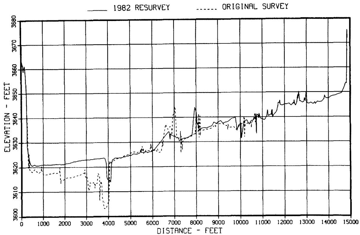
Figure 62. – Original and 1982 sedimentation range profiles, range 28.
