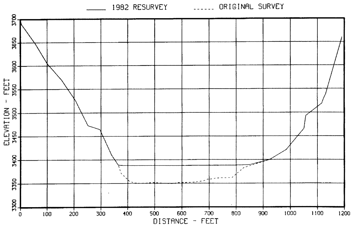
Figure 38. – Original and 1982 sedimentation range profiles, range 4.
