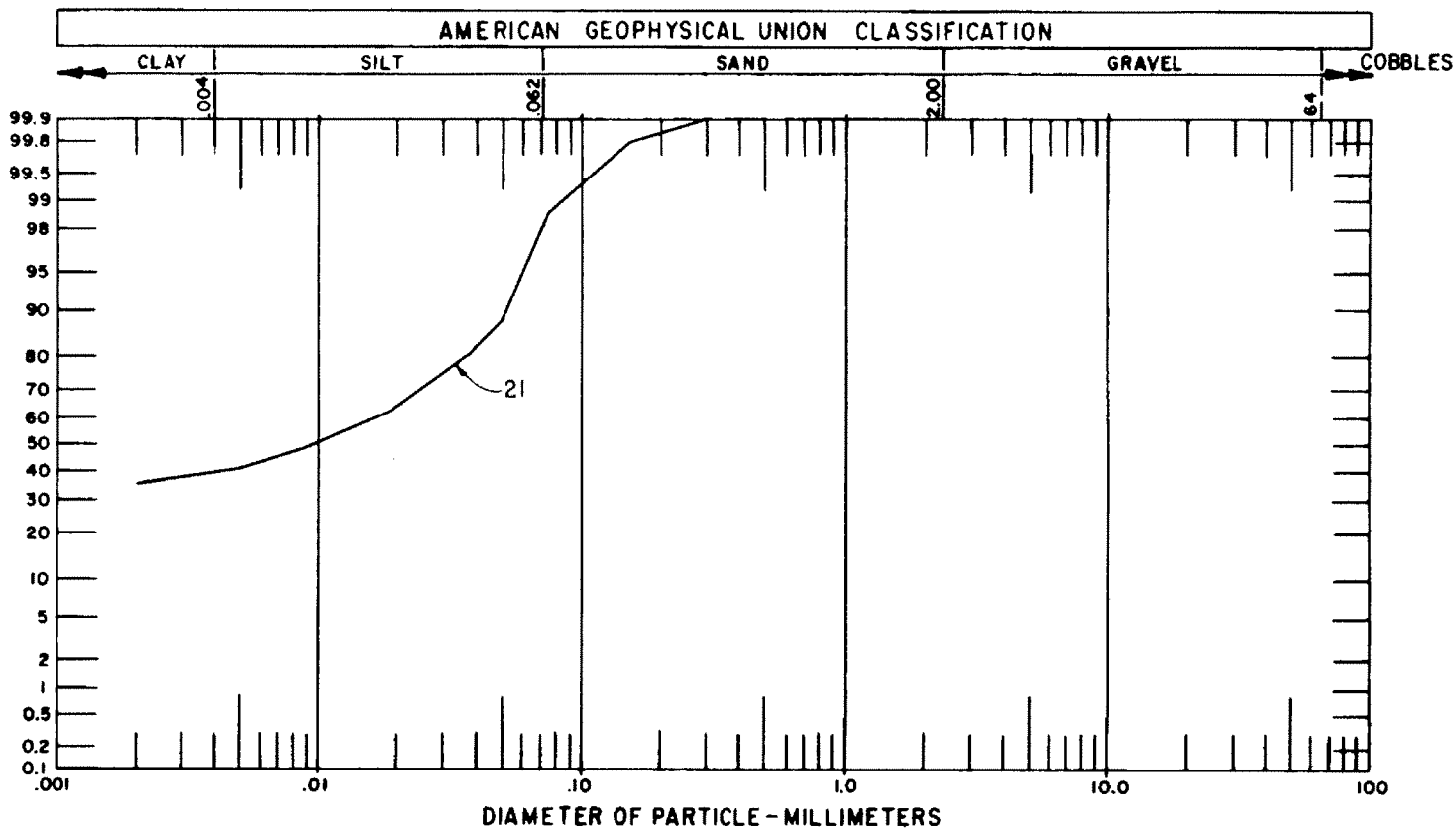
Figure 29. - Particle size analysis curve, range 34.
