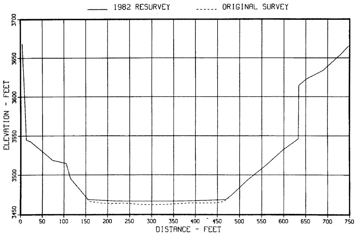
Figure 42. - Original and 1982 sedimentation range profiles, range 8.
