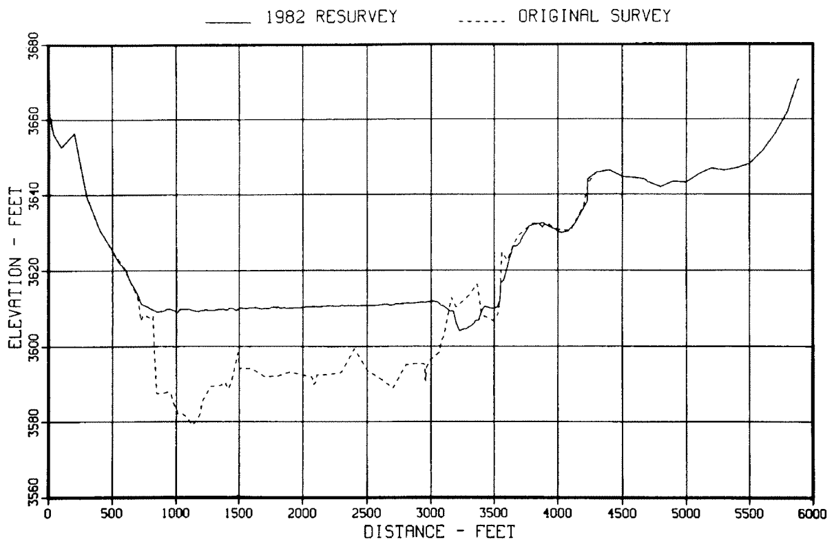
Figure 57. - Original and 1982 sedimentation range profiles, range 23.
