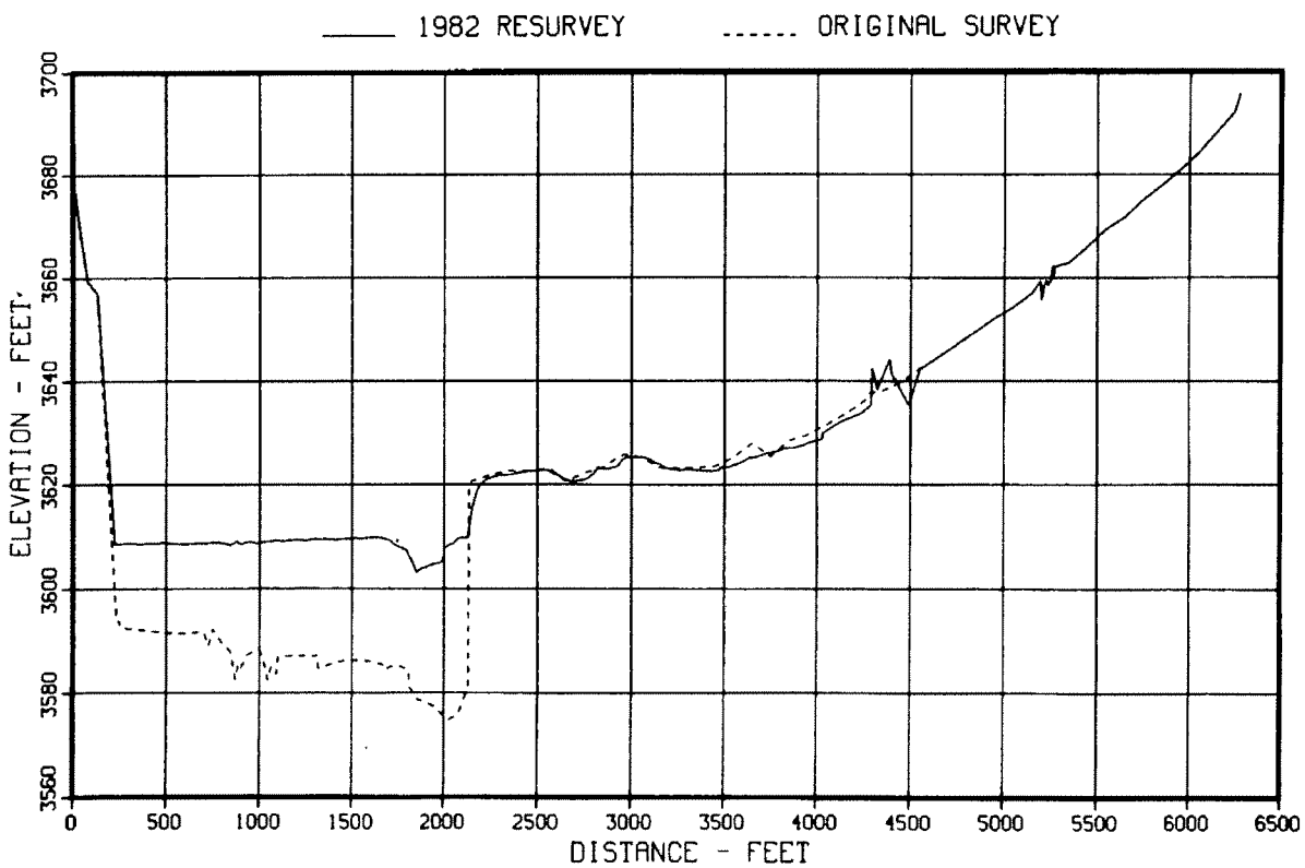
Figure 56. - Original and 1982 sedimentation range profiles, range 22.
