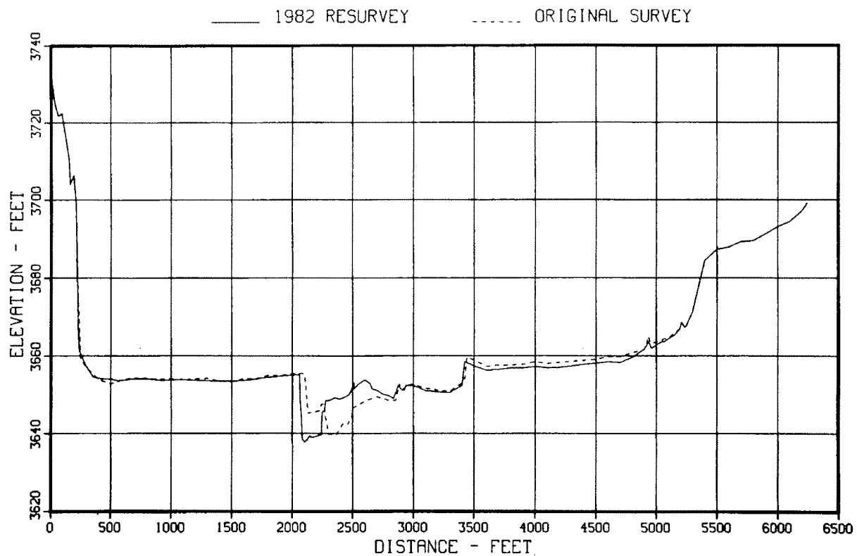
Figure 73. – Original and 1982 sedimentation range profiles, range 39.
