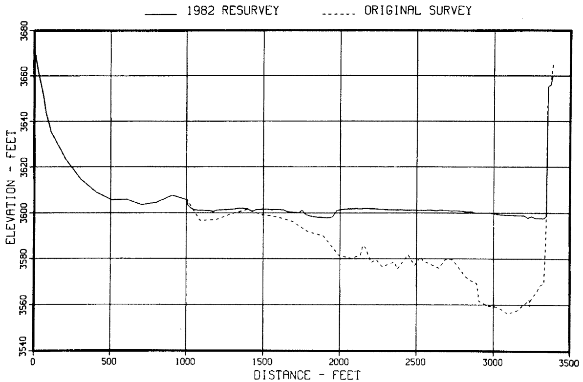
Figure 50. – Original and 1982 sedimentation range profiles, range 16.
