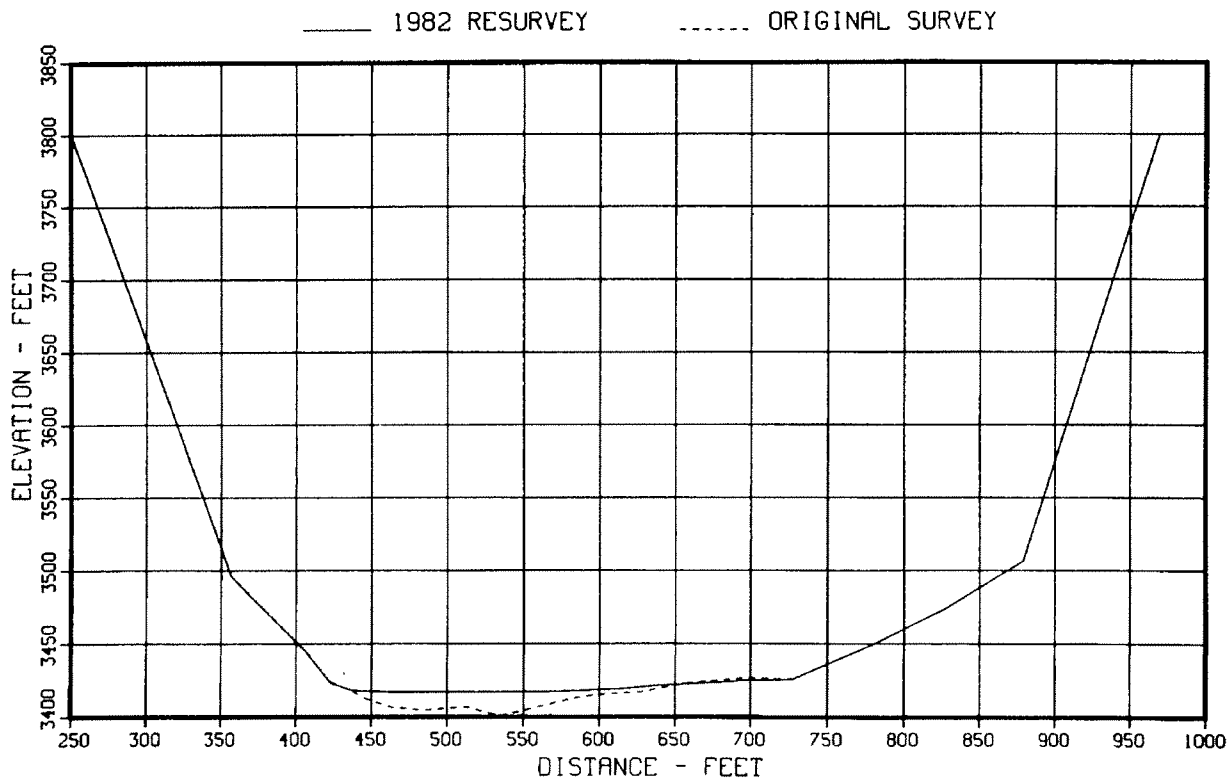
Figure 40. – Original and 1982 sedimentation range profiles, range 6.
