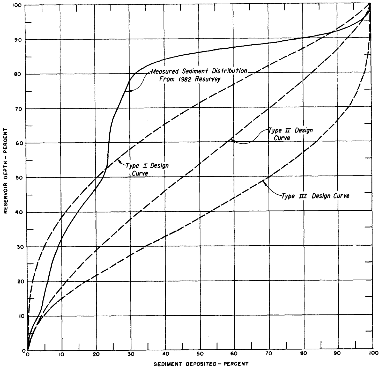
Figure 33. - Percent depth vs. percent sediment deposited.
