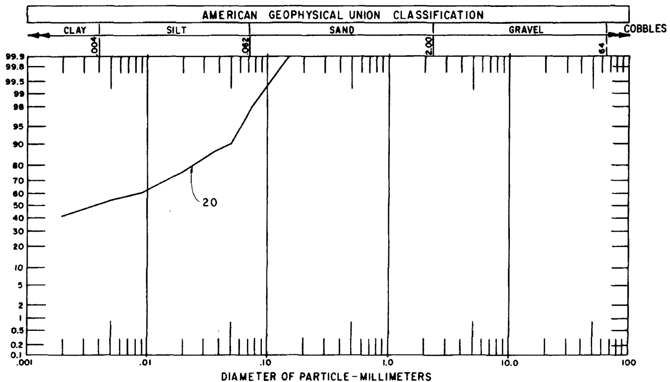
Figure 28. - Particle size analysis curve, range 33.
