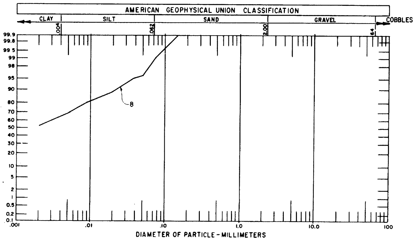
Figure 18. - Particle size analysis curve, range 18.
