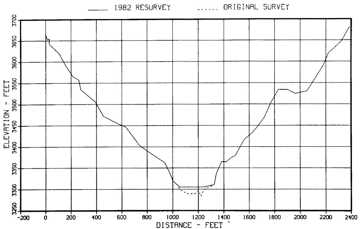
Figure 37. – Original and 1982 sedimentation range profiles, range 3.
