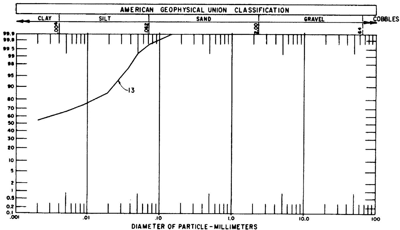
Figure 22. - Particle size analysis curve, range 22.
