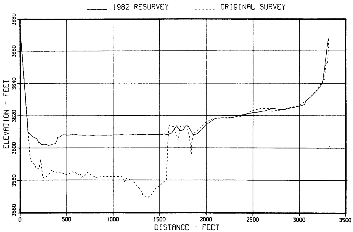
Figure 55. - Original and 1982 sedimentation range profiles, range 21.
