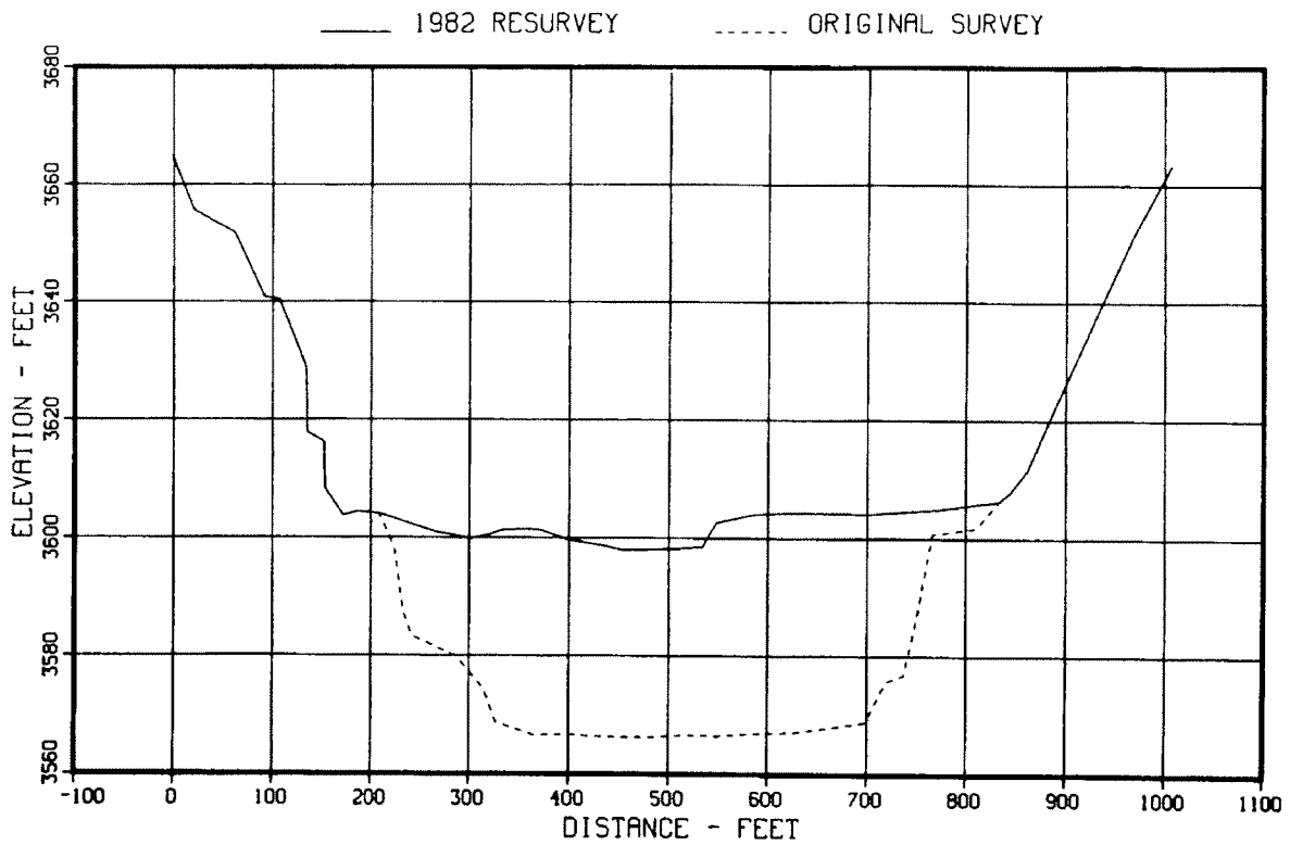
Figure 51. – Original and 1982 sedimentation range profiles, range 17.
