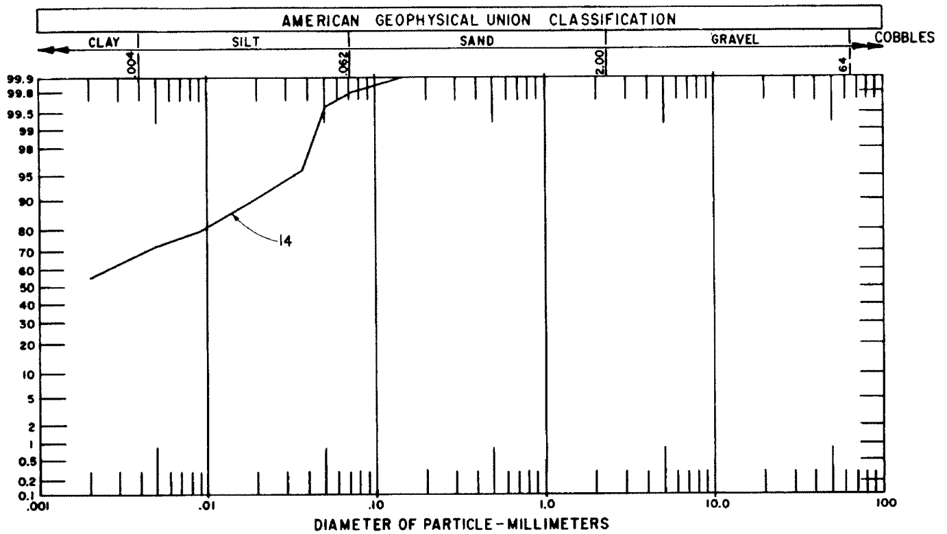
Figure 23. - Particle size analysis curve, range 23.
