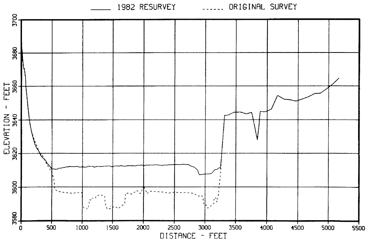
Figure 58. - Original and 1982 sedimentation range profiles, range 24.
