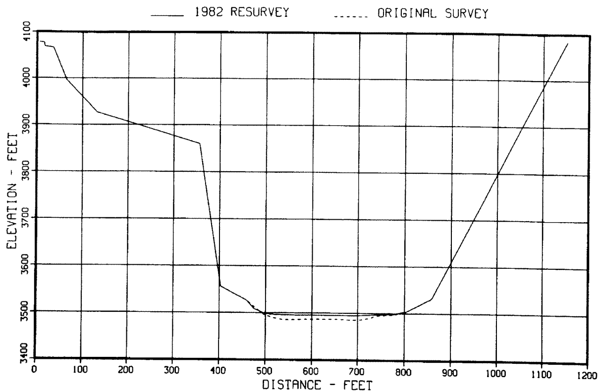
Figure 43. - Original and 1982 sedimentation range profiles, range 9.
