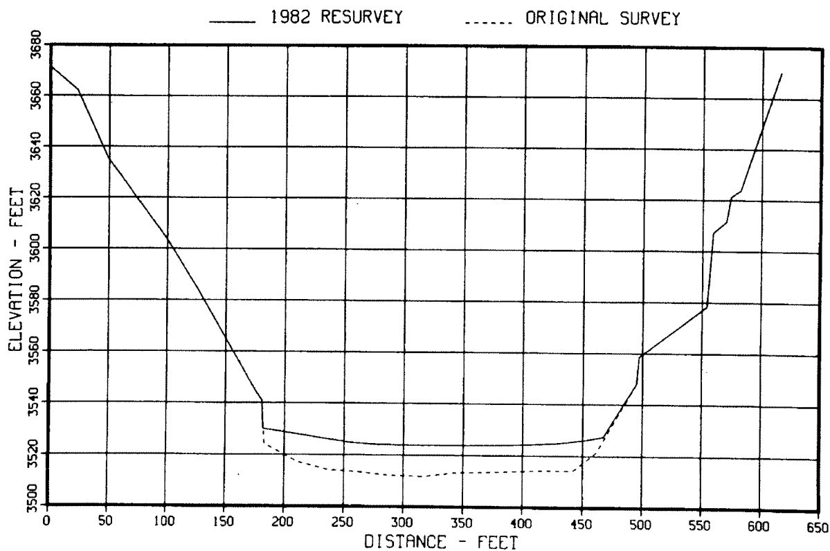
Figure 44. - Original and 1982 sedimentation range profiles, range 10.
