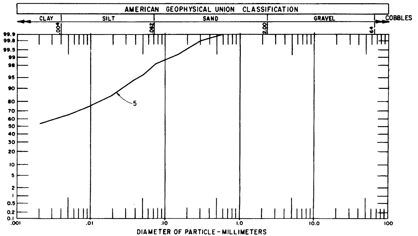
Figure 16. - Particle size analysis curve, range 16.
