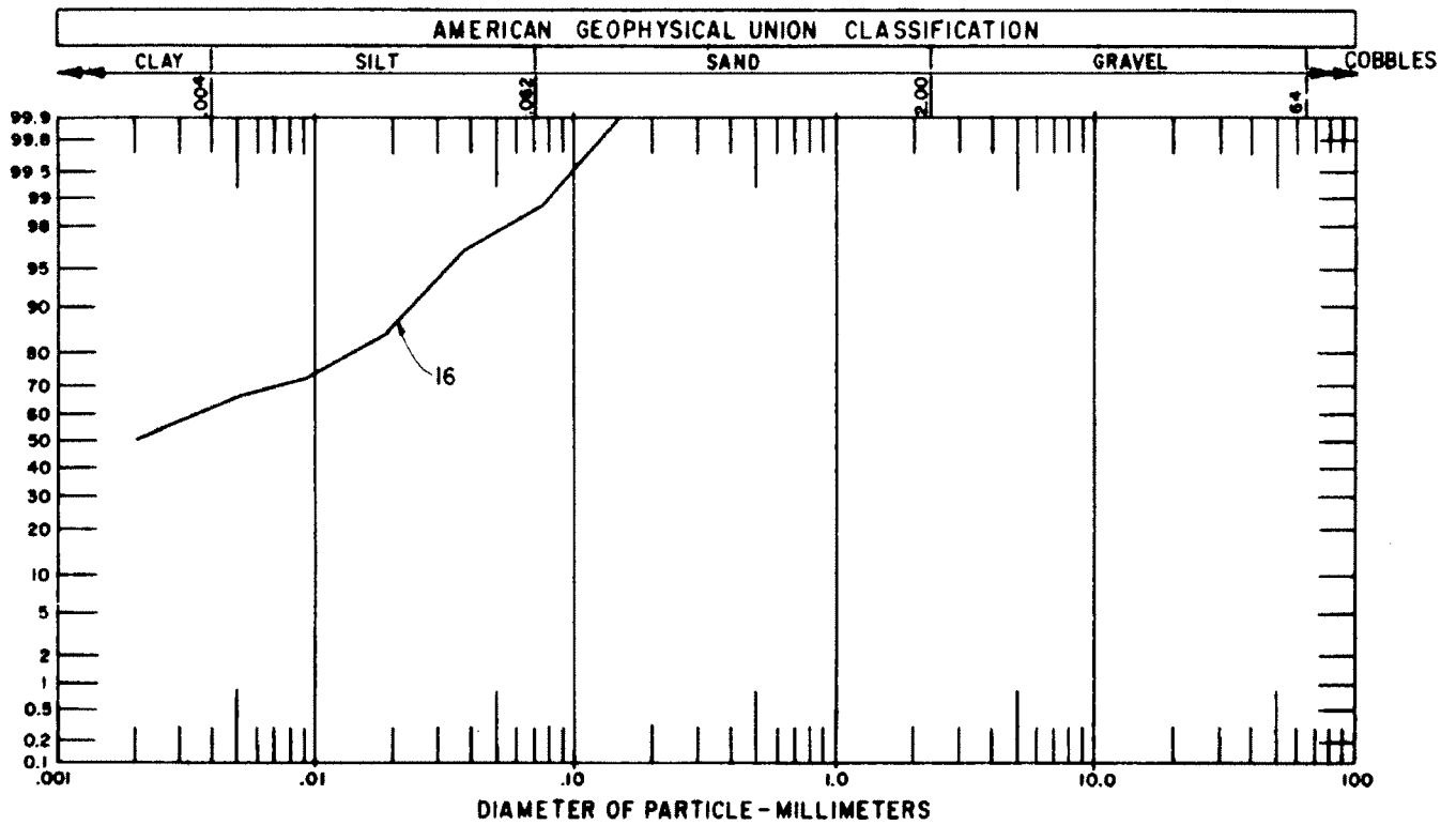
Figure 25. - Particle size analysis curve, range 25.
