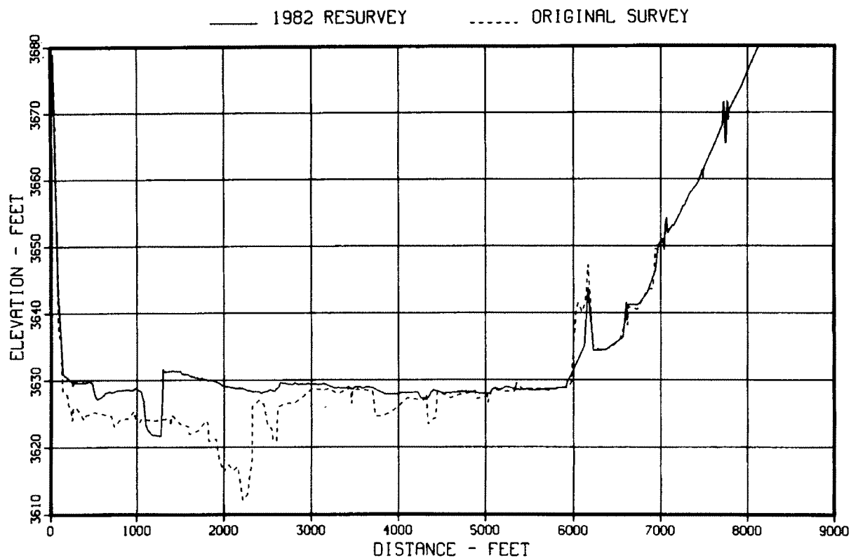
Figure 66. - Original and 1982 sedimentation range profiles, range 32.
