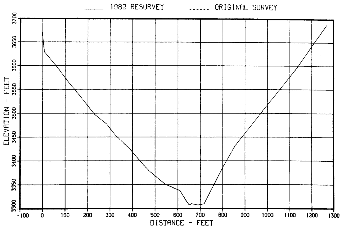
Figure 79. - Original and 1982 sedimentation range profiles, range 2A.
