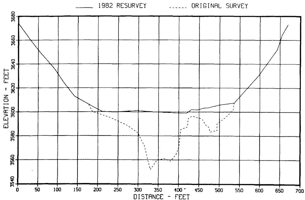
Figure 53. -- Original and 1982 sedimentation range profiles, range 19.
