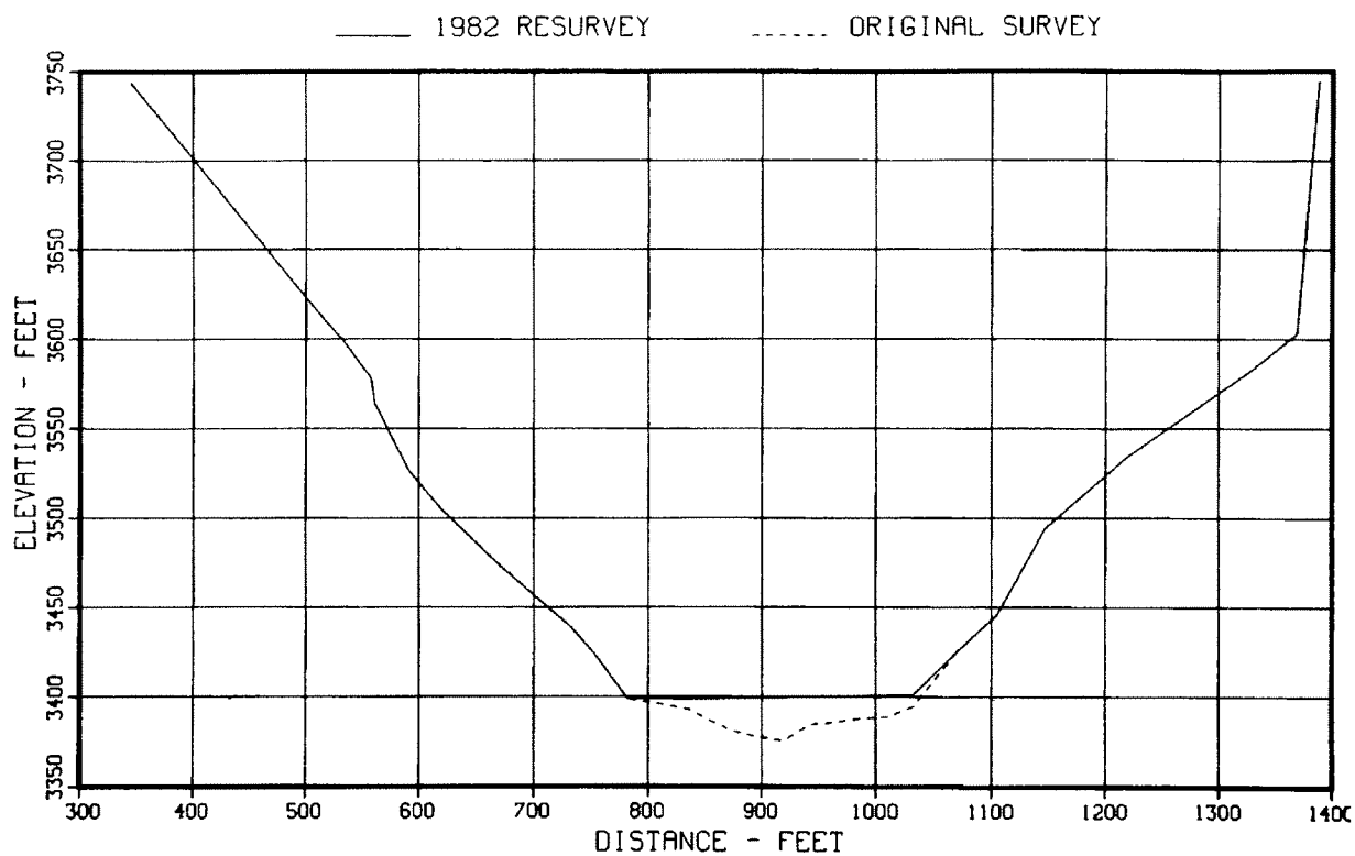
Figure 39. – Original and 1982 sedimentation range profiles, range 5.
