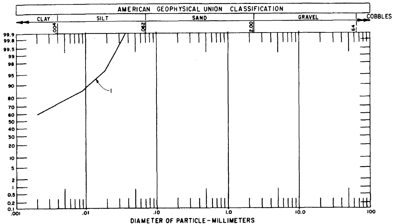
Figure 13. - Particle size analysis curve, range 13.
