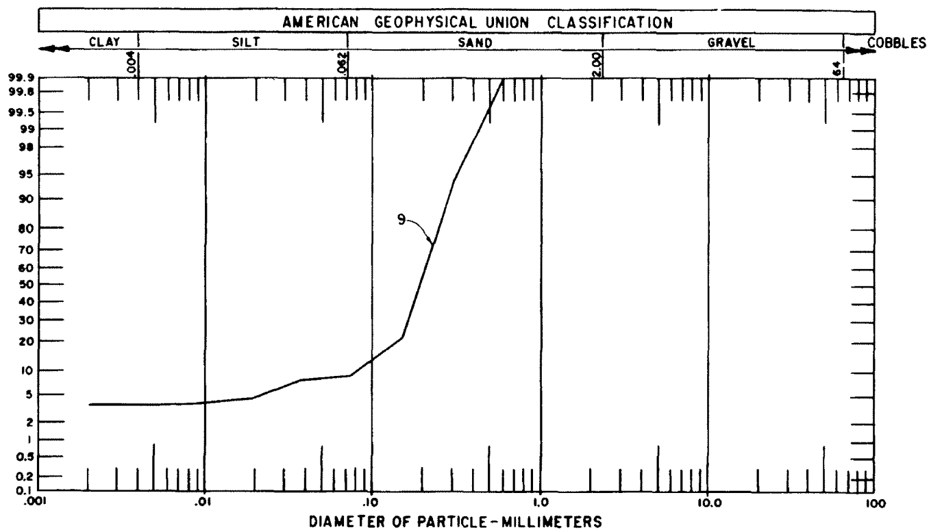
Figure 19. - Particle size analysis curve, range 19.
