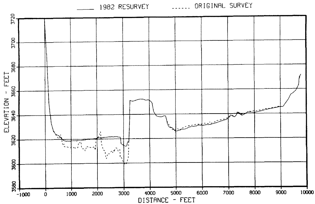
Figure 61. – Original and 1982 sedimentation range profiles, range 27.
