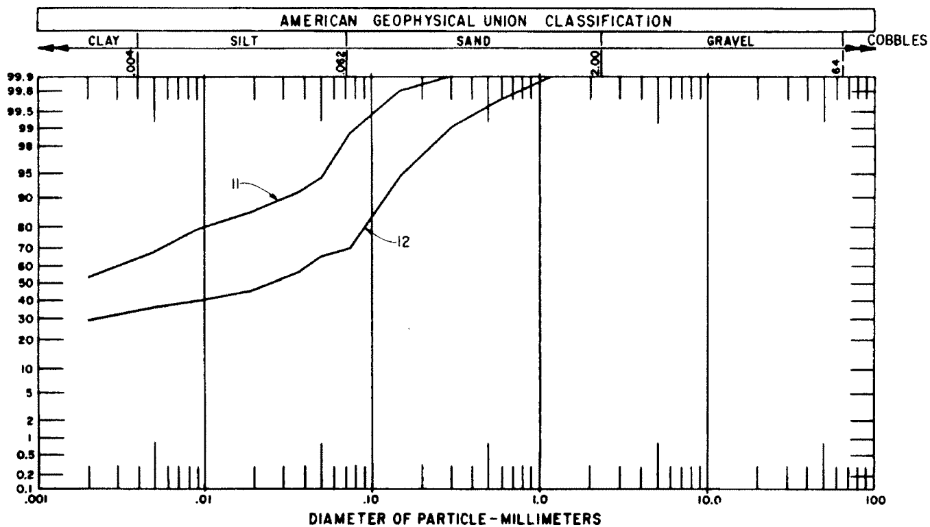
Figure 21. - Particle size analysis curves, range 21.
