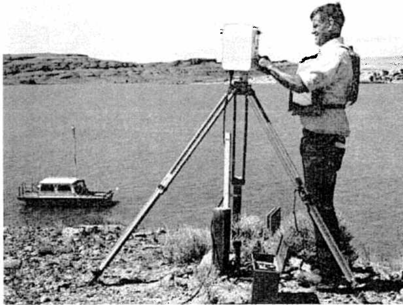
Figure 9. – Microwave receiver-transmitter at shore station. P801-D-80967
