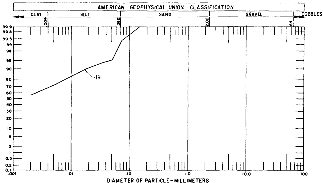
Figure 27. - Particle size analysis curve, range 32.
