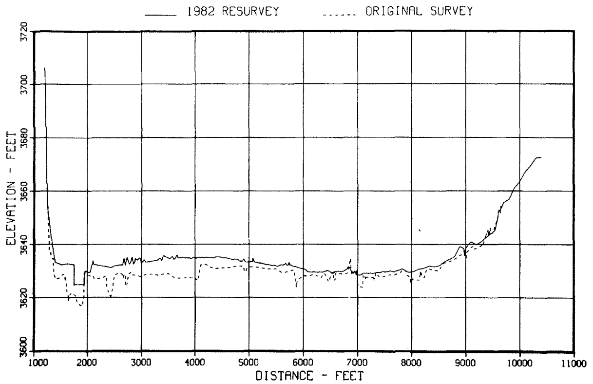
Figure 67. - Original and 1982 sedimentation range profiles, range 33.
