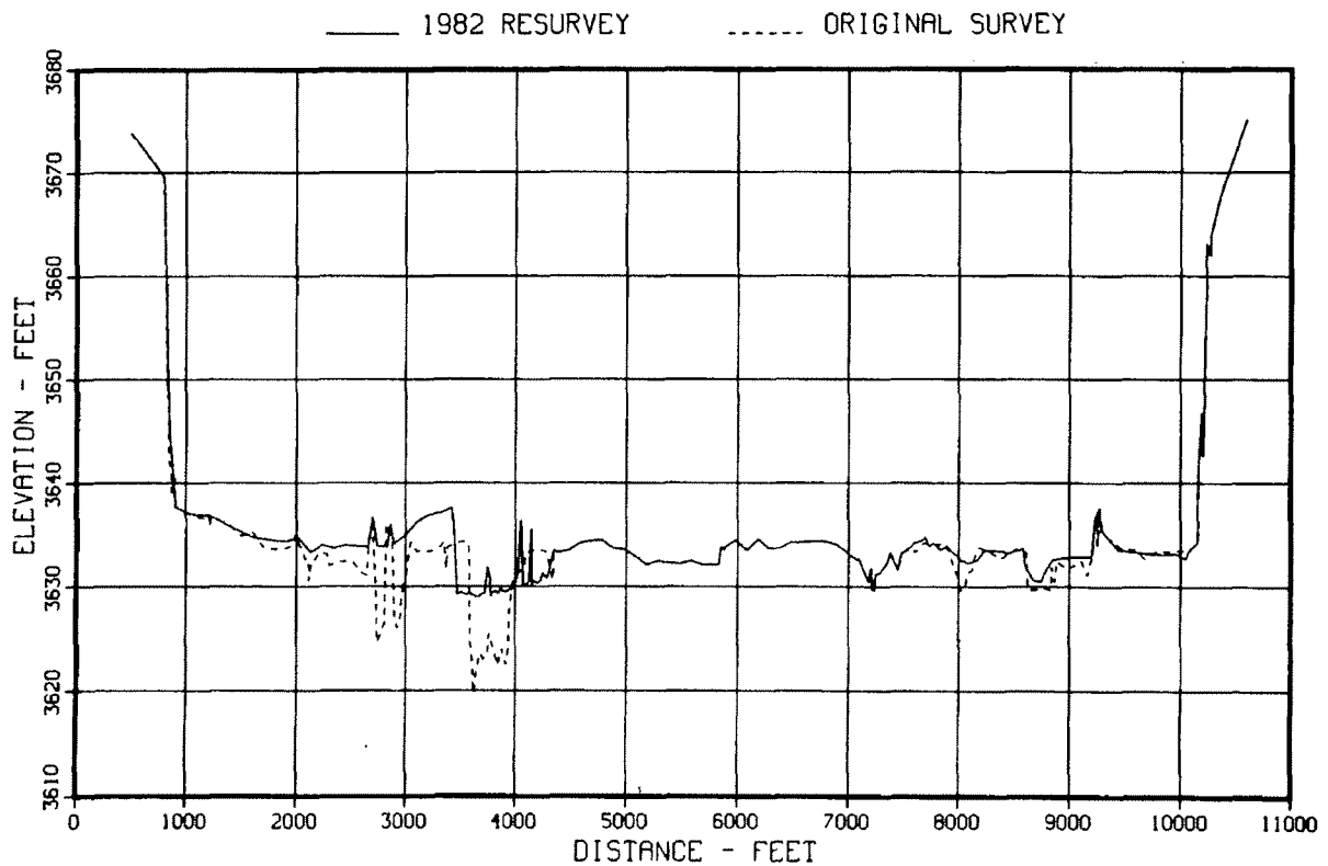
Figure 68. - Original and 1982 sedimentation range profiles, range 34.
