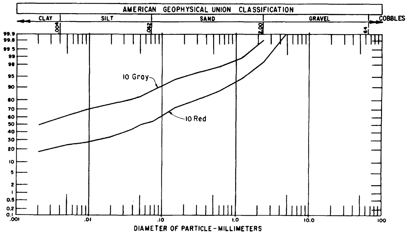
Figure 20. - Particle size analysis curves, range 20.
