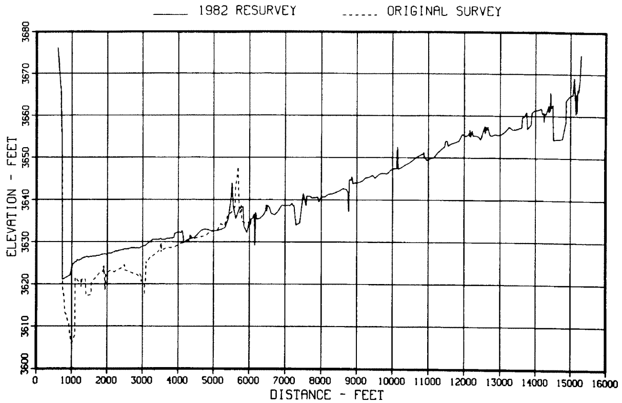
Figure 63. – Original and 1982 sedimentation range profiles, range 29.
