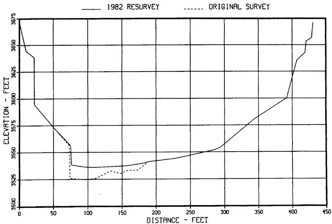
Figure 82. - Original and 1982 sedimentation range profiles, range 10A.
