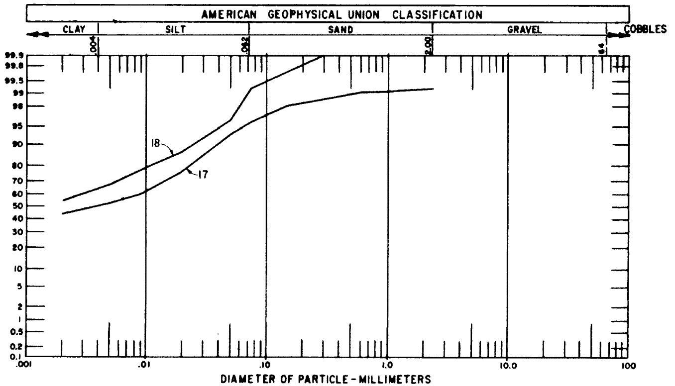
Figure 26. - Particle size analysis curves, range 31.
