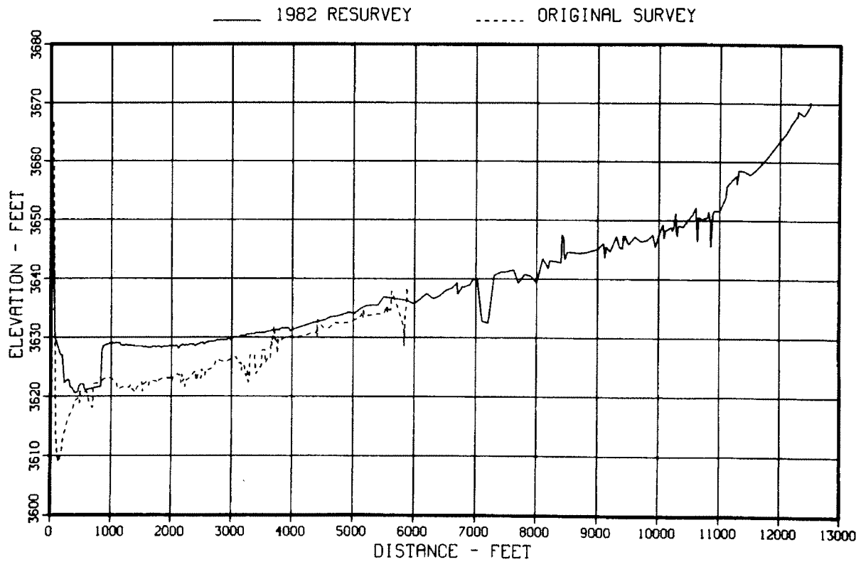
Figure 64. – Original and 1982 sedimentation range profiles, range 30.
